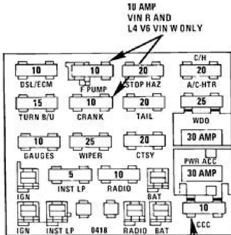
FRONT VIEW OF FUSE BLOCK
