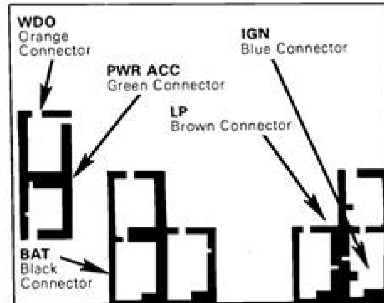
REAR VIEW OF FUSE BLOCK Connector Cavity Locations
